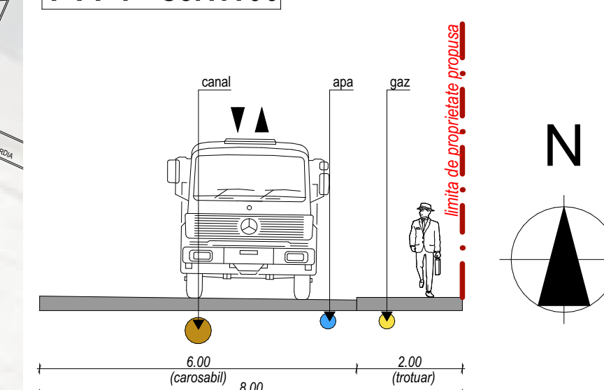
PTT 2 - sc.1:100
