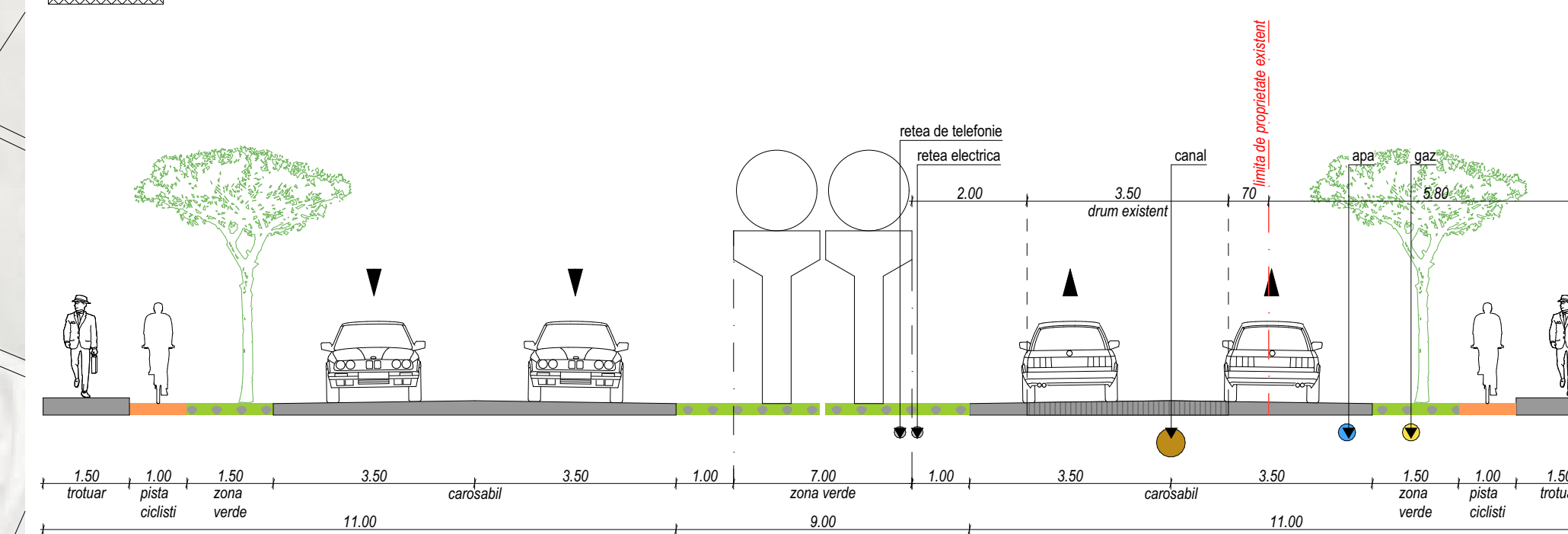
PTT 1 - sc.1:100
