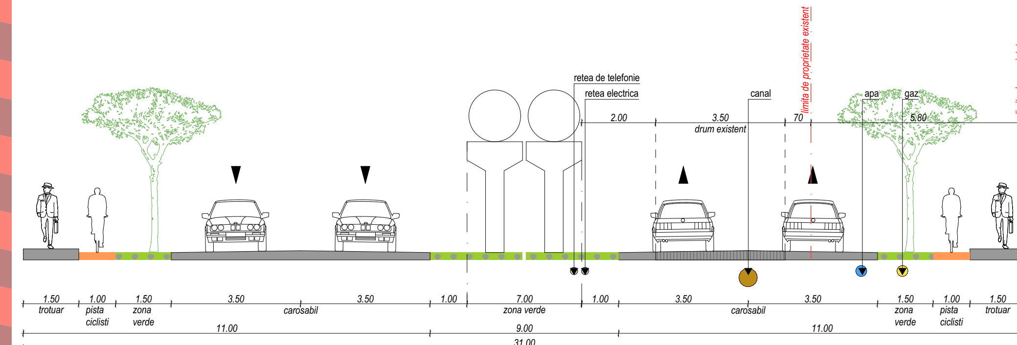
PTT 1 - sc.1:100
