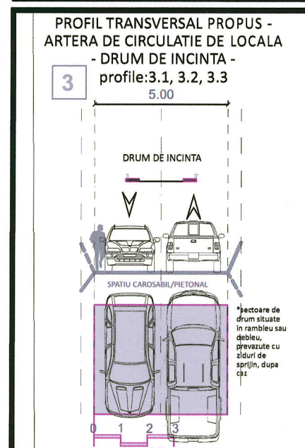
PROFILE DRUMURI - SCARA 1/200
