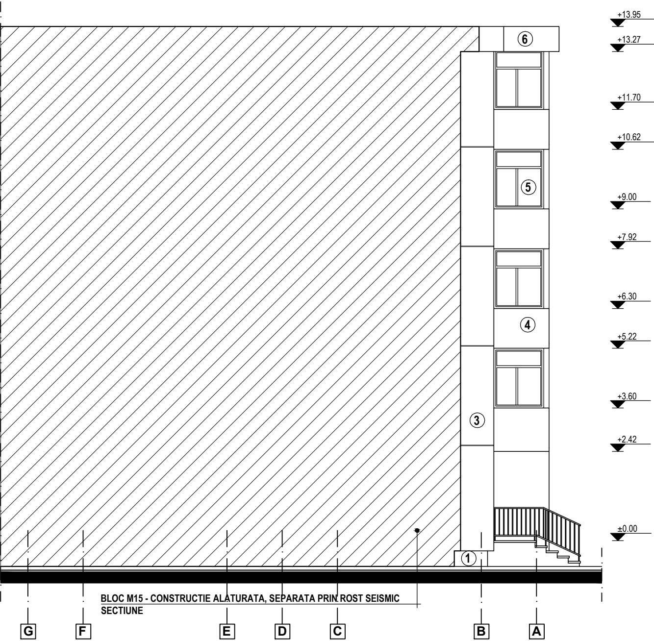
FATADA LATERALA STANGA
