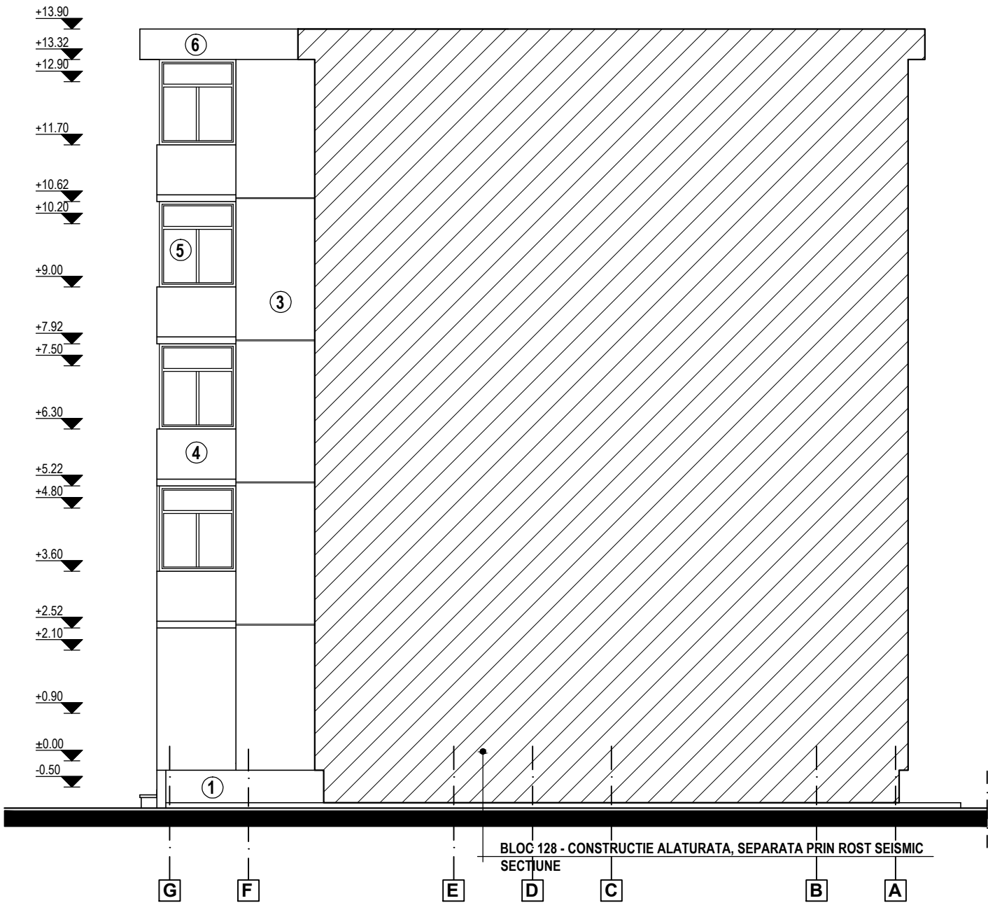
FATADA LATERALA STANGA
