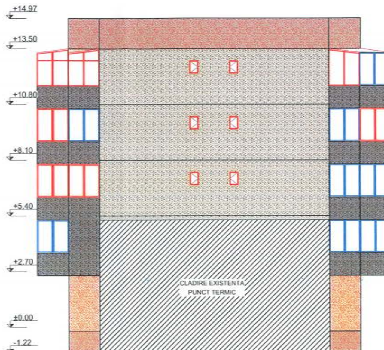
O21 Scara 1 FATADA LATERALA STANGA (EST)
