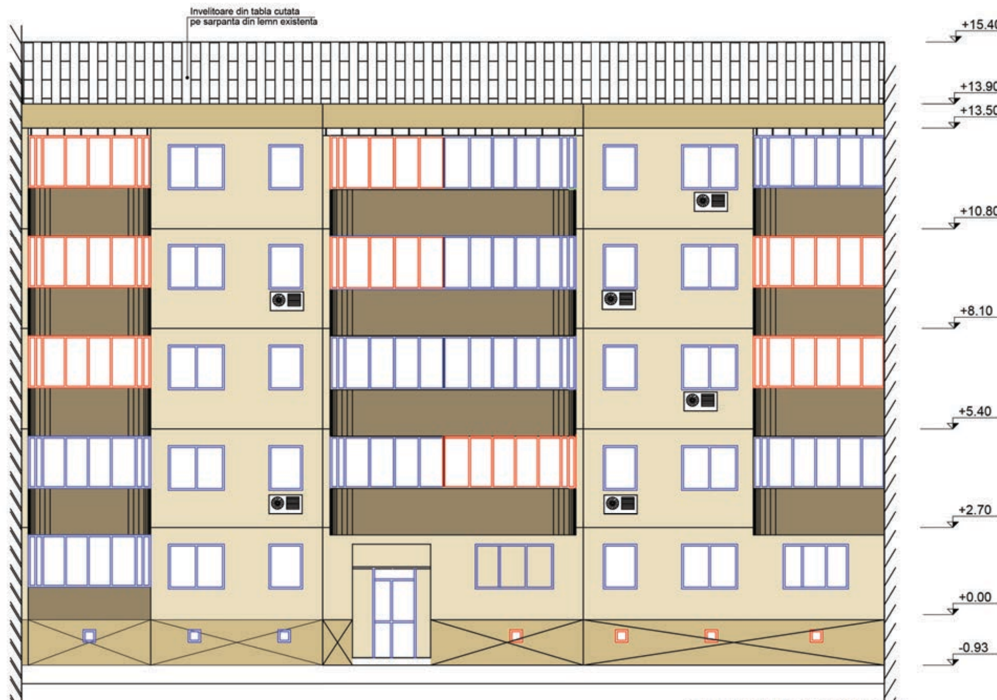
FATADA PRINCIPALA
