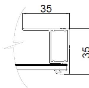
Frame Cross Section A-A
