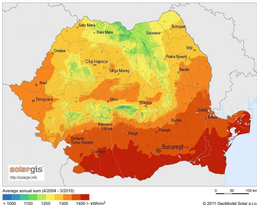
Global horizontal irradiation
