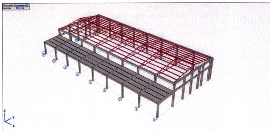
Model structural - propunere
