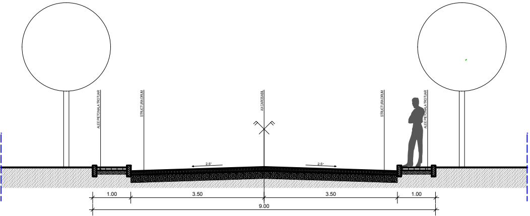
1-1 ALEE CAROSABILA - STR. PETROSANI SC. 1/100
